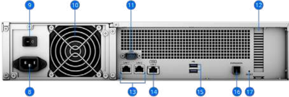
RS2423+ (Rear)
