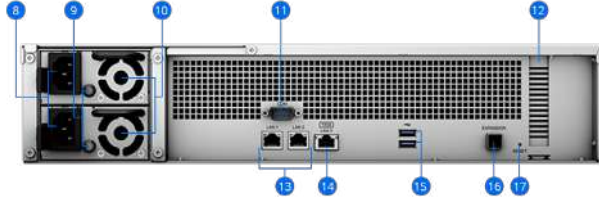
RS2423RP+ (Rear)
